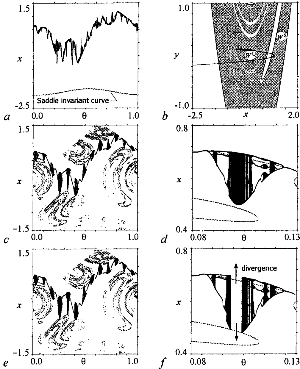
Fig. 3. a - The SNA on the threshold of crisis (route e ) at parameter values a=1.0925 , \epsilon=0.41 ; b - section of the phase space by plane \theta_0=0.41 at the same parameter values; black dots distributed along W^U denote projection of SNA from interval \theta \in [\theta_0 - 0.01, \theta_0 + 0.01] on the section. The rational approximation of level k=7 for c - the SNA and the ring-shaped unstable set on the threshold of crisis at a=1.067 , \epsilon=0.41 , and e - the «remnant» of SNA after crisis at a=1.069 , \epsilon=0.41 . The figures d and f represent the enlarged fragments of c and e , respectively
