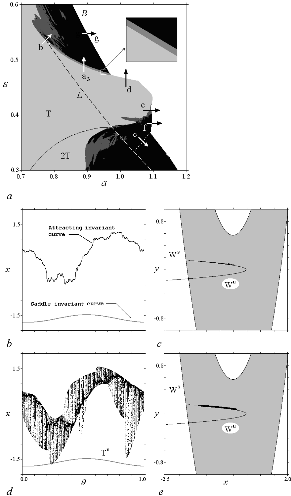
Fig. 1. a - The phase diagram of the system (1) (here and thereafter we set the parameter b=0.1 ). Regular, chaotic, SNA, and divergence regimes are shown in light gray, black, gray (or dark gray), and white, respectively. To show the existence of intermittent SNA (gray), a small segment near (a, \varepsilon)=[0.95, \varepsilon^*] is magnified. Solid line denotes the doubling bifurcation of invariant curve. Due to interaction with the ring-shaped unstable sets born when passing the dashed line L , different dynamical transition such as intermittency (route a ), interior (routes b and c ), and basin-boundary (routes d , e and f ) crises can occur. b - The smooth attractor (black) and saddle invariant curve (gray) at a=0.95 and \varepsilon=0.4761 ; c - the section of the phase space by plane \theta_0=0.2 at the same parameter values; the basin of attractor is shown in gray; the black dot embedded into unstable manifold W^U is a section of smooth attractor. d - SNA at a=0.95 and \varepsilon=0.476149 ; e - the plane \theta_0=0.2 at the same parameter values. Black dots distributed along W^U denote projection of SNA from the interval \theta \in [\theta_0 - 0.01, \theta_0 + 0.01] on the plane
